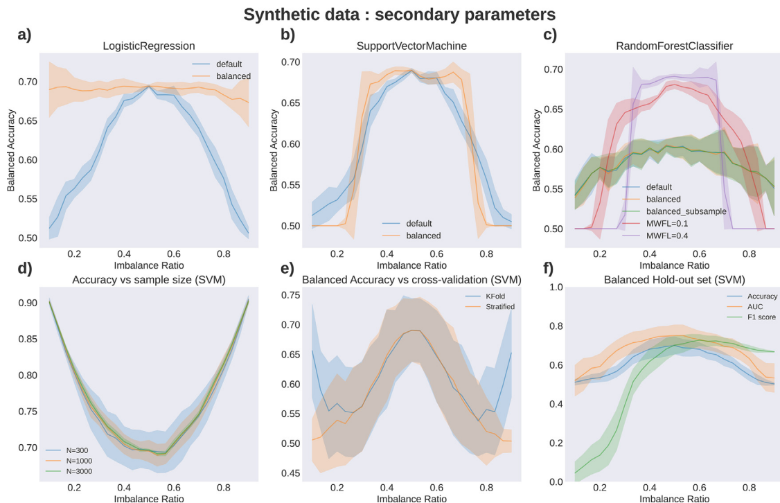
Fig. 3. These examples follow the same principle as previous analysis (Fig 2), expanding on the effect of secondary parameters and hyperparameter tuning on the robustness to imbalance. (a-c) Exploration of the effect of hyperparameters on classifier robustness against imbalance. Each line represents a certain hyperparameter setting (Section 2.3.1) (d) The effect of sample size on robustness to class imbalance using an SVM and Acc. (e) The impact of cross-validation scheme on robustness to class imbalance (BAcc and SVM). (f) Performance metrics on a balanced hold-out set using an SVM trained on different ratios of imbalance. BAcc is not shown here as it is equivalent to Acc for balanced data. Solid lines show the performance over different class imbalance ratios, averaged over 10 initializations. Colored areas represent the respective standard deviation.
